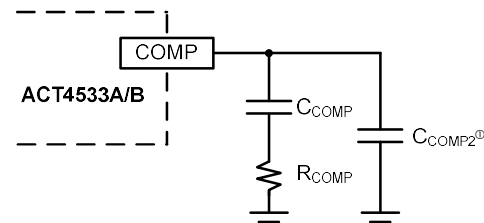
Figure 5: Stability Compensation
