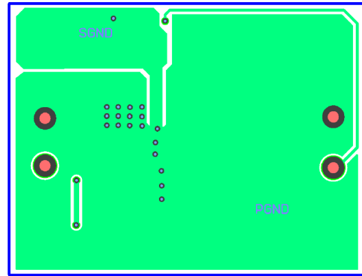
Figure 8: PCB Layout
